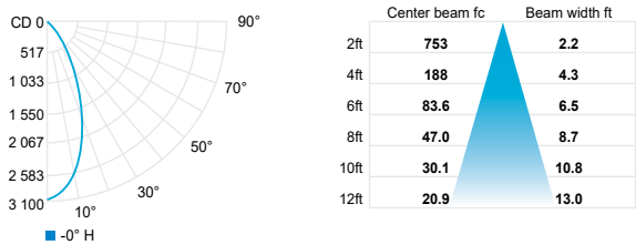
Flood BO 57° (3000K, Full spectrum)
