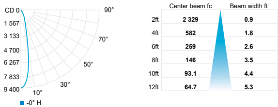
Spot BO 25° (3000K, Full spectrum)
