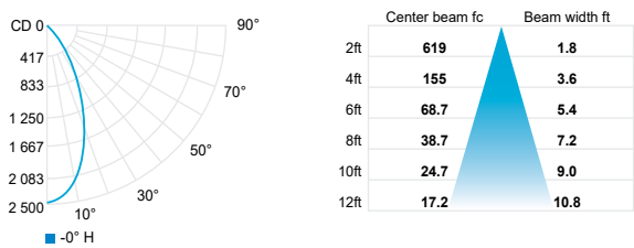
Flood BO 49° (3000K, Full spectrum)
