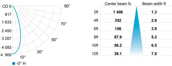
Narrow flood BO 36° (3000K, Full spectrum)
