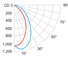
3000K - HO - 80 CRI - 45.5W - Wall washer
