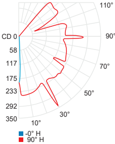
HO 360° blade effect (3000K,80CRI)
