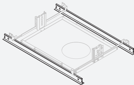
Hanger bars suitable for Grid ceiling
