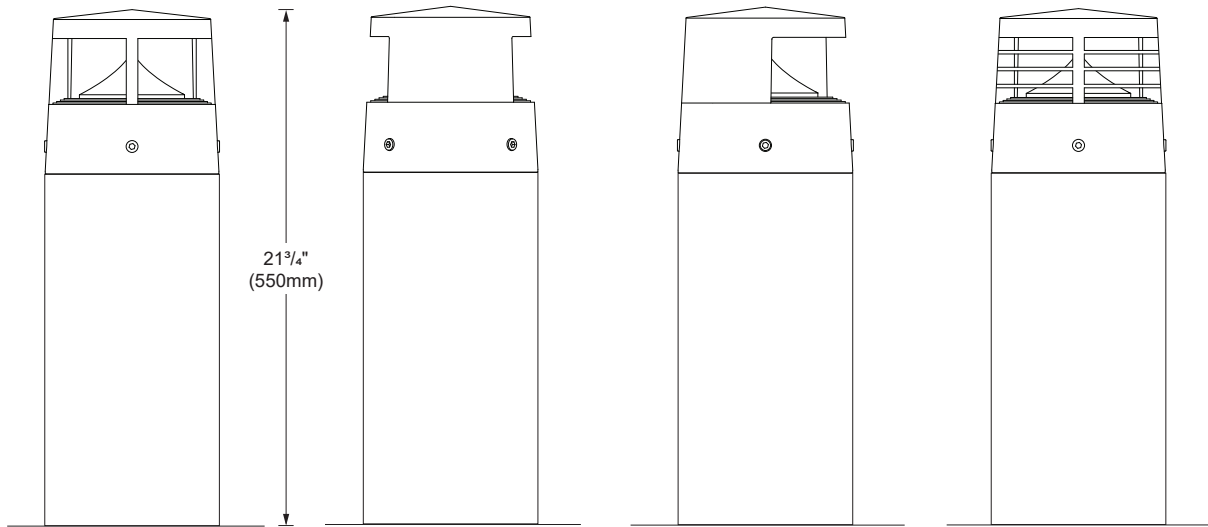
SIDE VIEW
