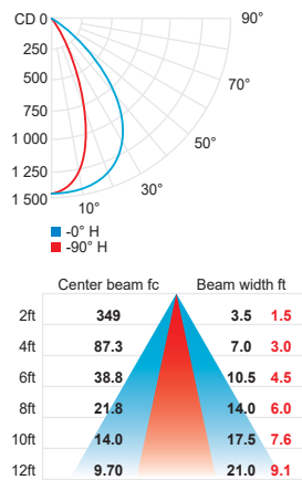
Wide flood oval tran. (3000K, 92CRI)
