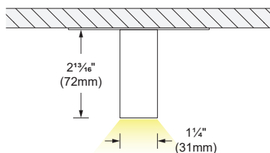
COMPACT PROFILE (3464)
