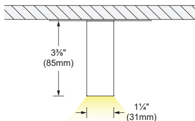
HIGH PROFILE (3454)
