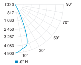
Wide flood 47° (3000K, 92CRI)
